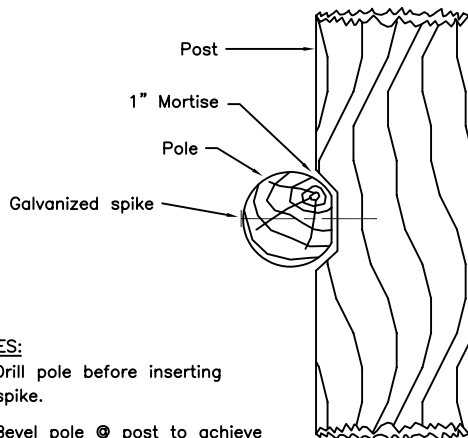
POST AND POLE CONNECTION
